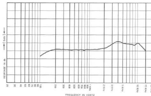
Figure 1 - Frequency Response
